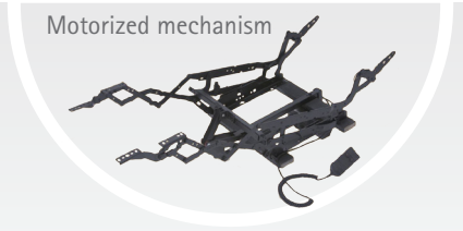
Three-way mechanism
